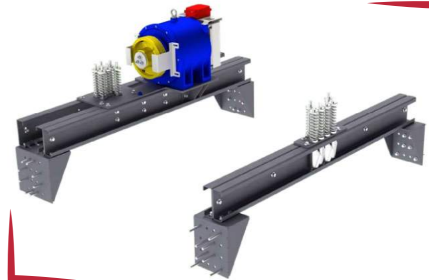
MRL. MACHINE MOTOR FRAME
