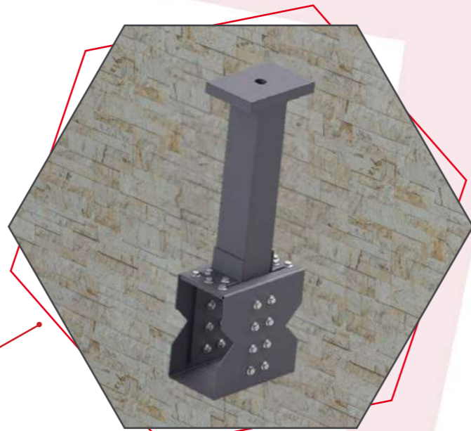
PISTON BASE
