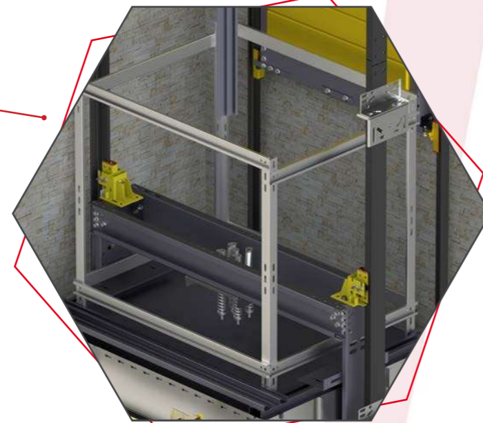
CAR BALUSTRADE
