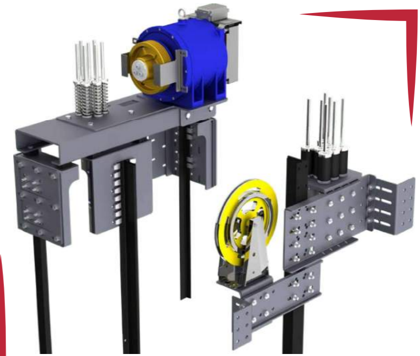
MRL. MACHINE MOTOR FRAME
